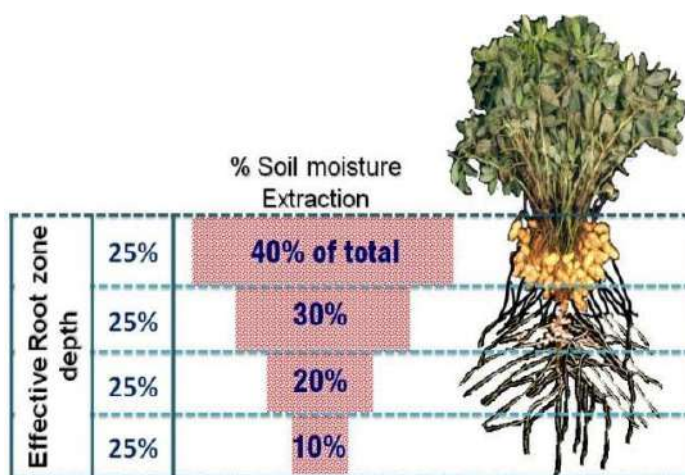
Fig 7.1: Basic soil moisture extraction pattern
